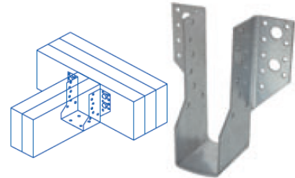
Special non-standard widths available to order. **Safe working load when fully nailed & bolted.
